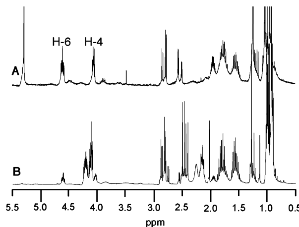
Figure 5. ^1\text{H} NMR comparison of (A) enzymatically generated triketide lactone 10 and (B) synthetic 5:1 mixture of 9 and 10 .
