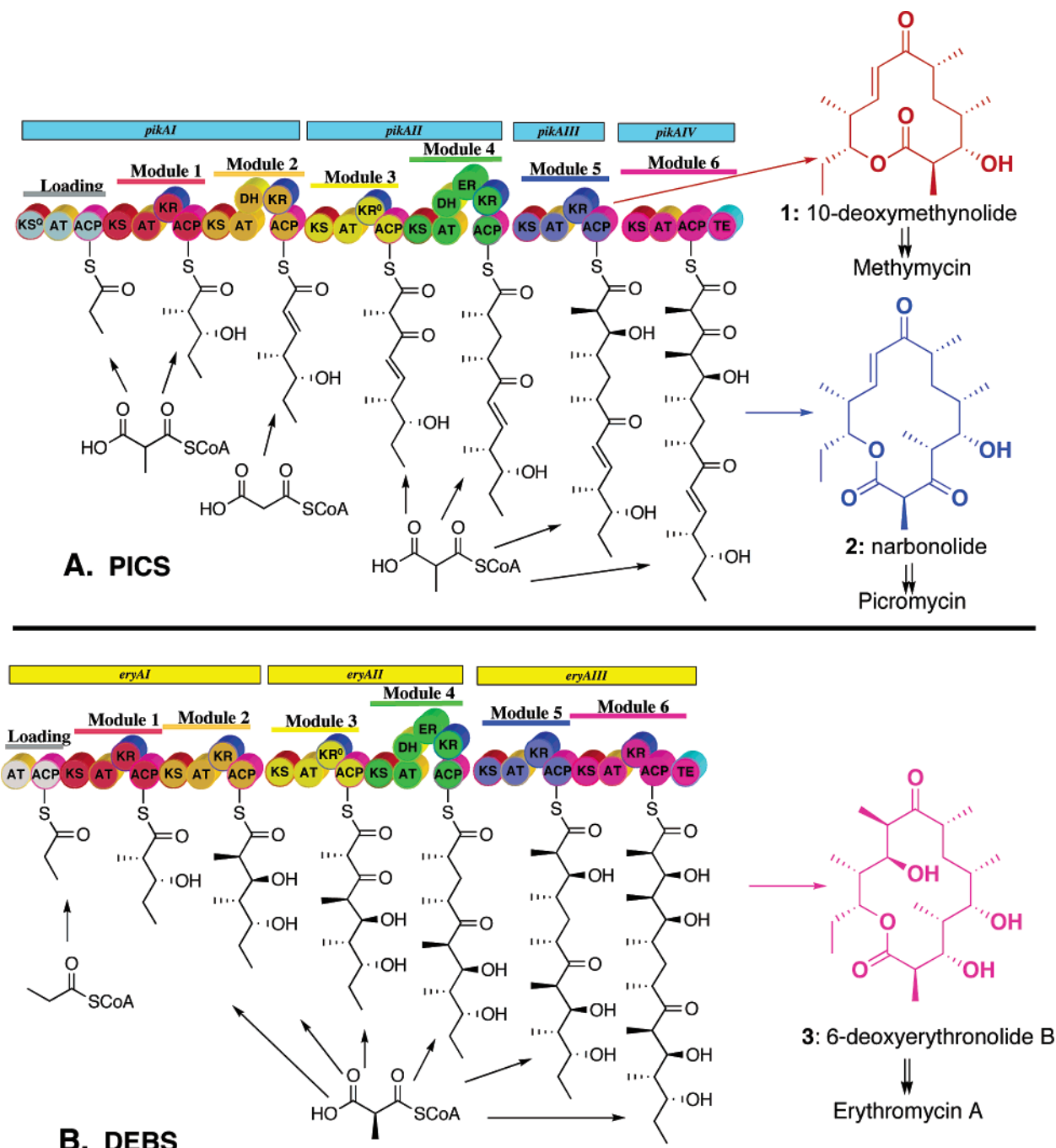
Figure 1. Modular organization of (A) picromycin/methymycin synthase (PICS) and (B) 6-deoxyerythronolide B synthase (DEBS). In addition to the three core catalytic domains—the ketosynthase (KS), acyl transferase (AT), and acyl carrier protein (ACP) domains—individual modules carry specific combinations of auxiliary ketoreductase (KR), dehydratase (DH), and enoylreductase (ER) domains. Loading tri- or didomains prime module 1 of each synthase with the propionyl starter unit and dedicated thioesterase (TE) domains cyclize the mature polyketide with release of the corresponding macrolide aglycone.
