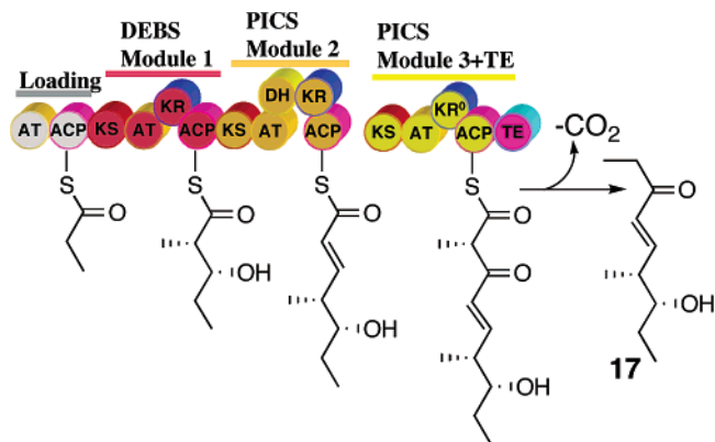
Scheme 5. In Vivo Generation and Processing of the Unsaturated Triketide by a Hybrid DEBS/PICS Trimodular PKS Containing PICS Modules 2 and 3
