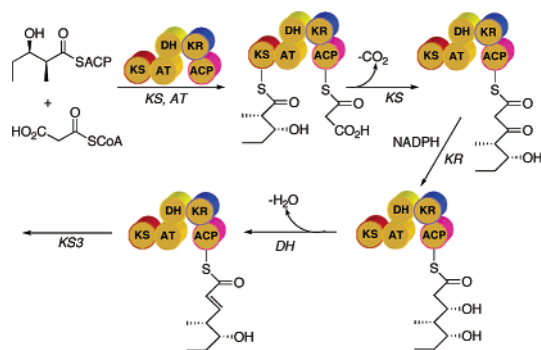
Figure 2. Sequence of reactions catalyzed by PICS module 2.
