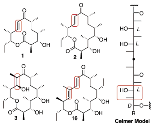
Figure 9. Celmer model of macrolide structure and stereochemistry, illustrating homologous sites of dehydration.
