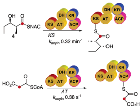
Scheme 4. Acylation of PICS Module 2 by Diketide 4 and Malonyl-CoA
