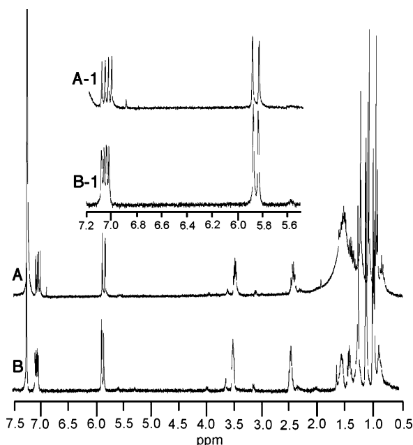
Figure 4. ^1\text{H} NMR comparison of (A) enzymatically generated triketide acid 5 and (B) synthetic 5 .
