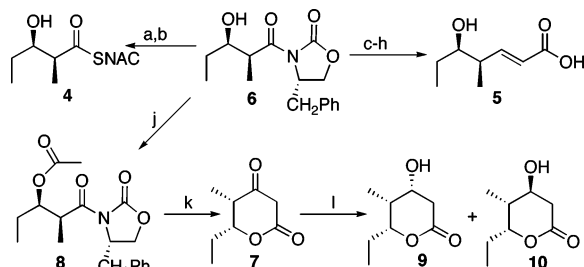
Scheme 1. Synthesis of Diketide 4 and Triketides 5 , 10 , and 7 a
